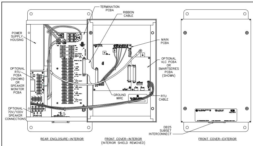
Figure 1. ICS Page/Party® Remote Subset Handset/Speaker Amplifier Station with available options (AC Version shown)
