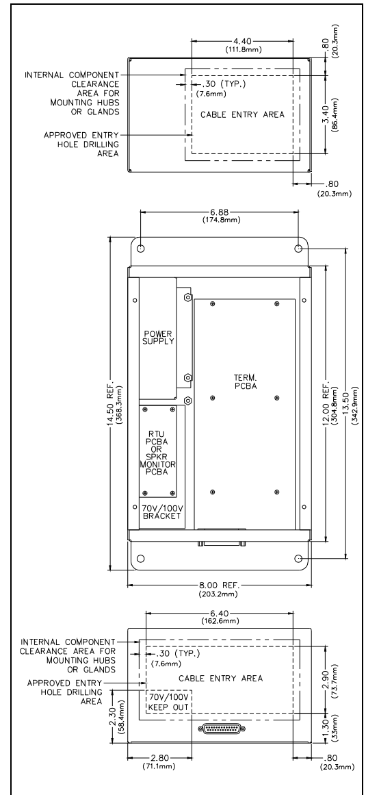
Figure 2. Suggested wire entry locations
