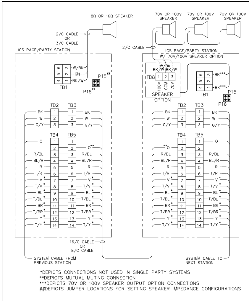
Figure 3. Typical installation wiring configuration
